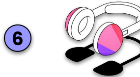
Playback audio
