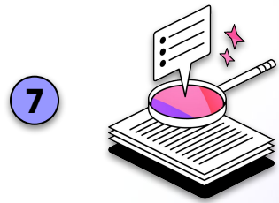
Edit notes
