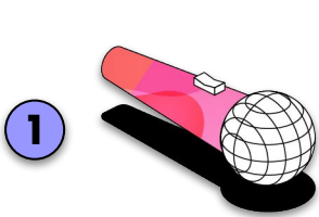
Record audio
