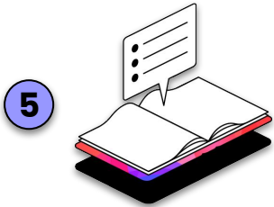
Transcribe & outline
